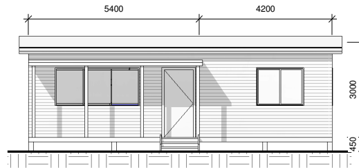
2 Front Elevation 1 : 100
