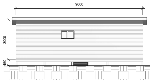
4 Rear Elevation 1 : 100
