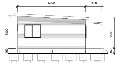
3 Side Elevation 1 : 100
